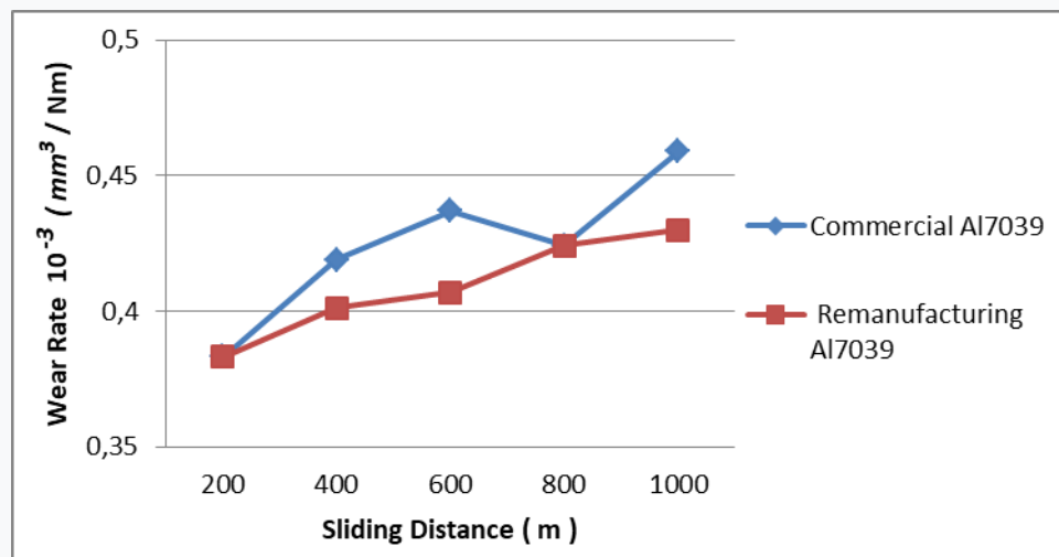
Figure 14. Wear rate graph of commercial and remanufactured Al7039 samples
