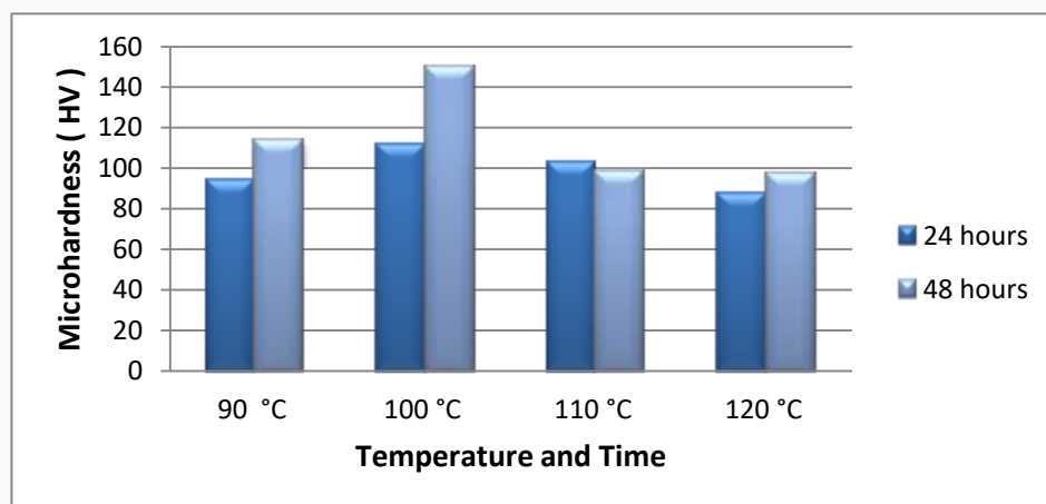
Figure 11. Micro hardness values of samples subjected to artificial aging at different temperatures and waiting times
