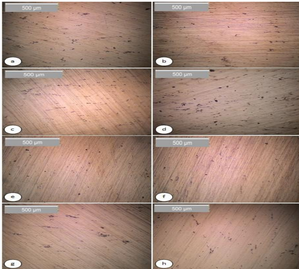
Figure 10. Microstructure images of samples aged at 24 and 48 hours respectively for artificial aging at different temperatures.
