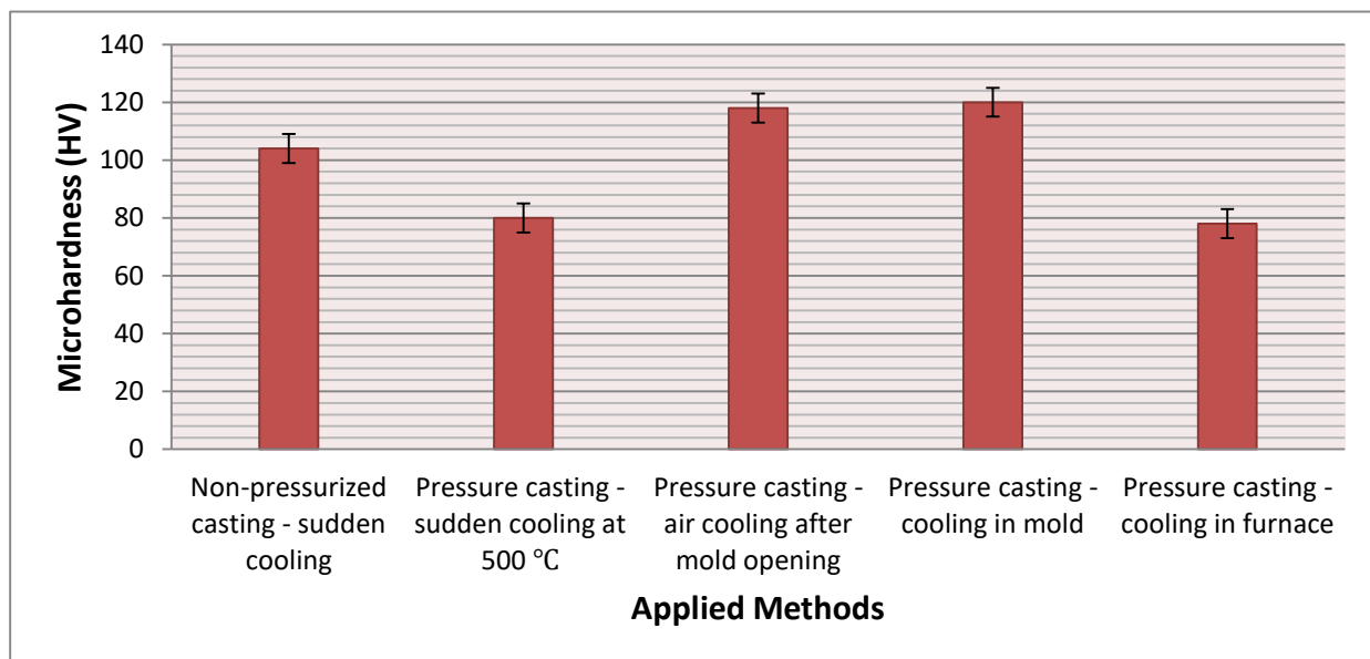
Figure 5. Hardness values of the obtained samples
