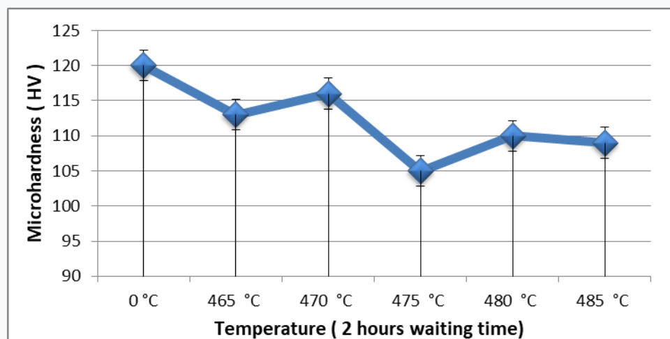
Figure 8. Hardness values of samples subjected to quenching after 2 hours of waiting at the specified temperatures.
