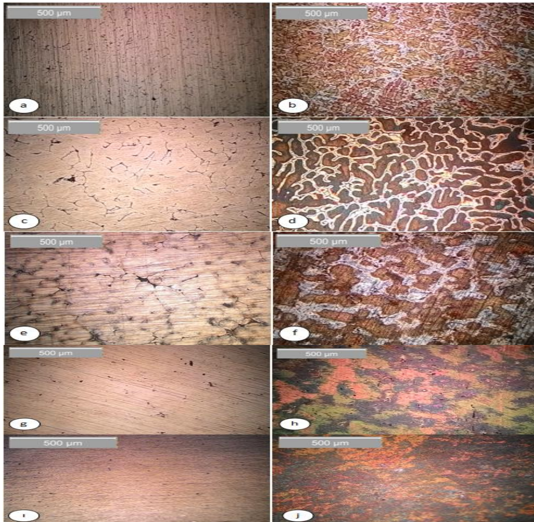
Figure 4. Microstructure images after casting a-b) non-pressurized casting - sudden cooling, c-d) pressure casting - sudden cooling at 500 °C, e-f) pressure casting - air cooling after mold opening, g-h) pressure casting - cooling in mold, i-j) pressure casting - cooling in furnace
