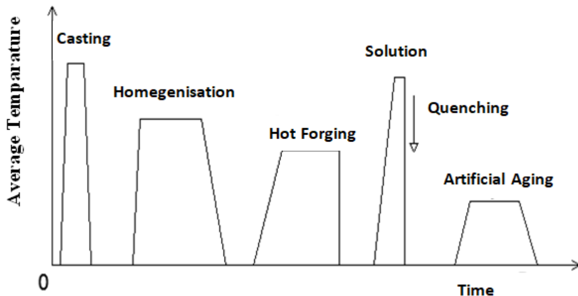
Figure 1. Production stages of 7xxx series aluminum alloys
