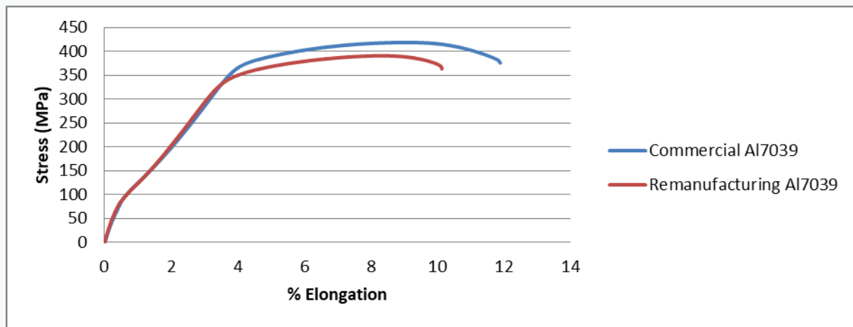
Figure 13. Tensile test graph of commercial and remanufactured Al7039 samples
