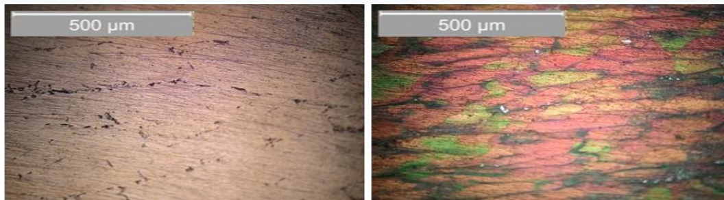
Figure 6. After the hot forging, microstructure images ( Respectively Keller and Weck solution )
