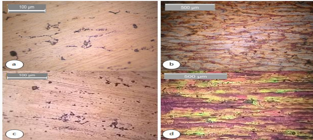
Figure 12. a-b) Microstructure image after artificial aging process, c-d) Microstructure image of commercial Al 7039 sample
