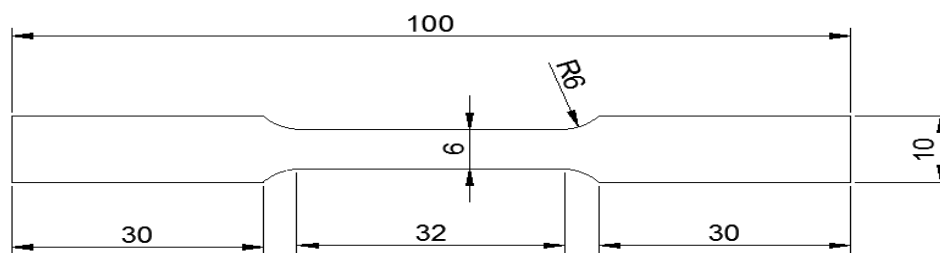
Figure 3. Tensile test sample dimensions (mm)
