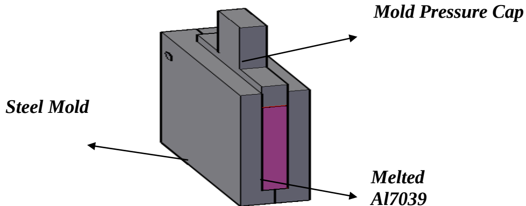
Figure 2. Pressure application after casting.
