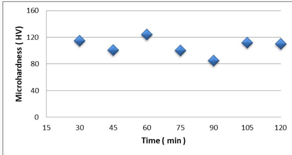
Figure 9. Micro hardness values of the samples which were taken into solution at 480 °C for different periods and subjected to quenching.
