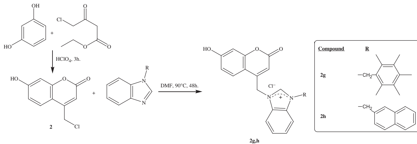
Scheme 2. Synthesis of 7-hydroxy coumarin bearing benzimidazolium salts ( 2g, h ).
