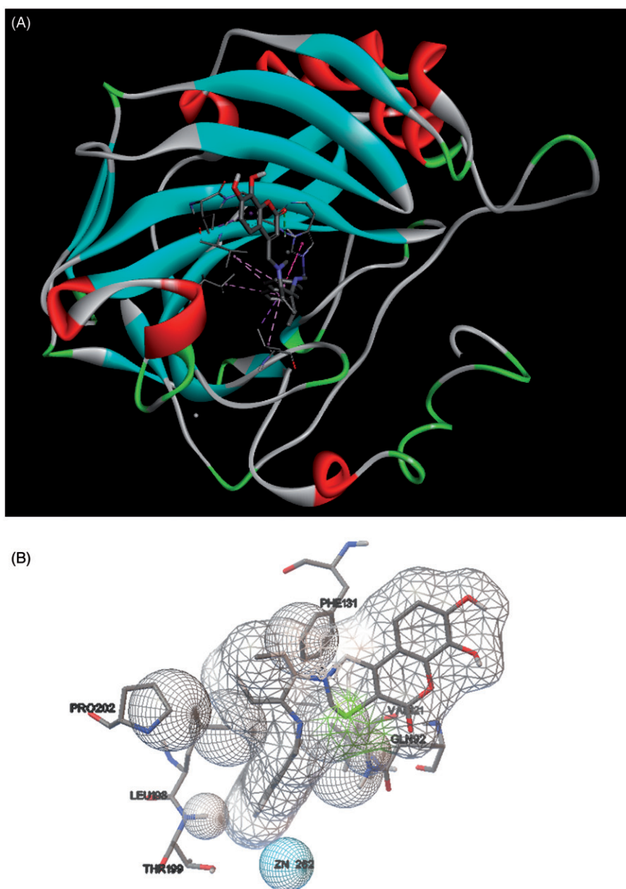
Figure 1. Docking of compound 3j within the hCA II active site. (A) Discovery Studio 4.0 Client images and (B) ADT images.
