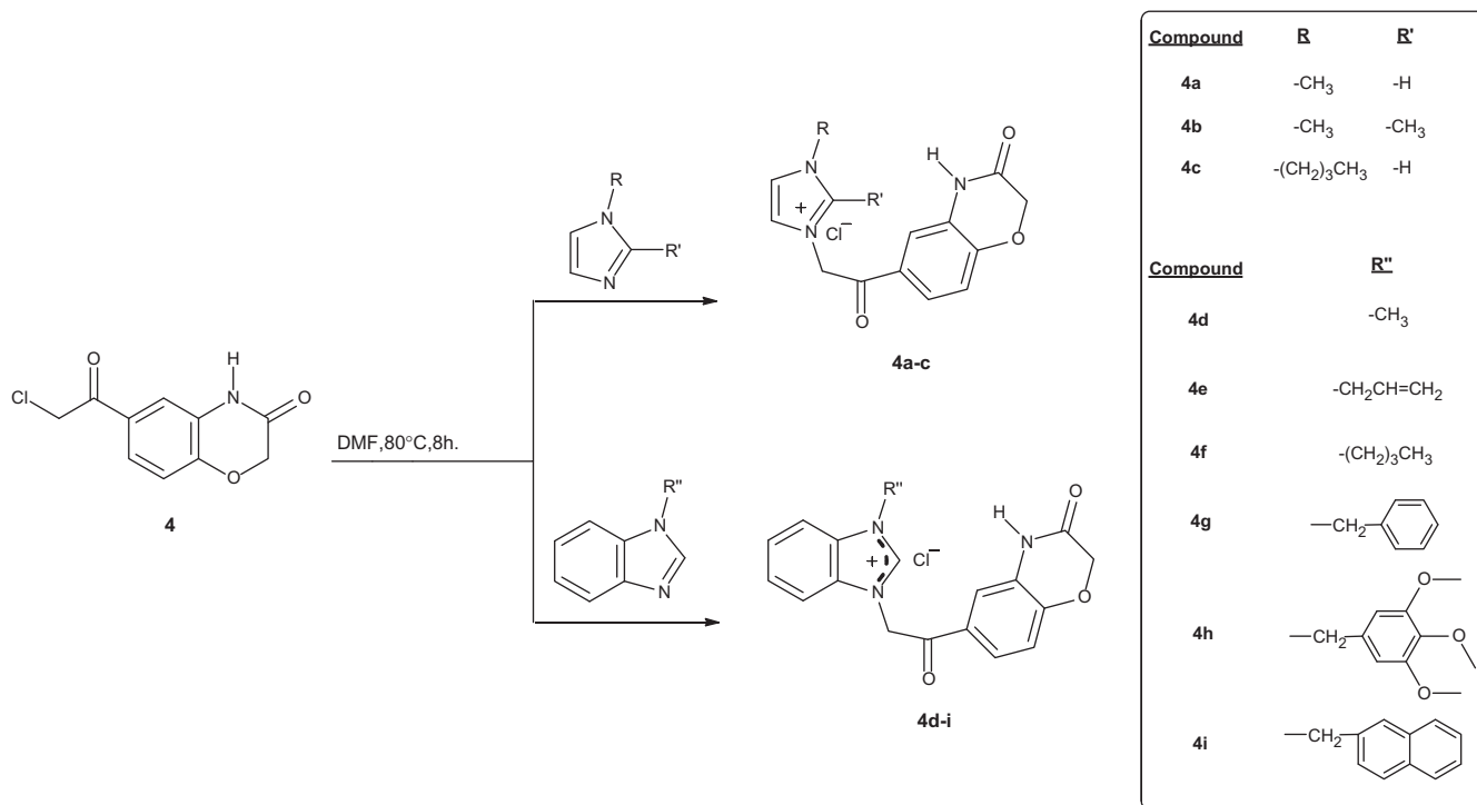
Scheme 4. Synthesis of benzoxazinone bearing imidazolium and benzimidazolium salts ( 4a-i ).
