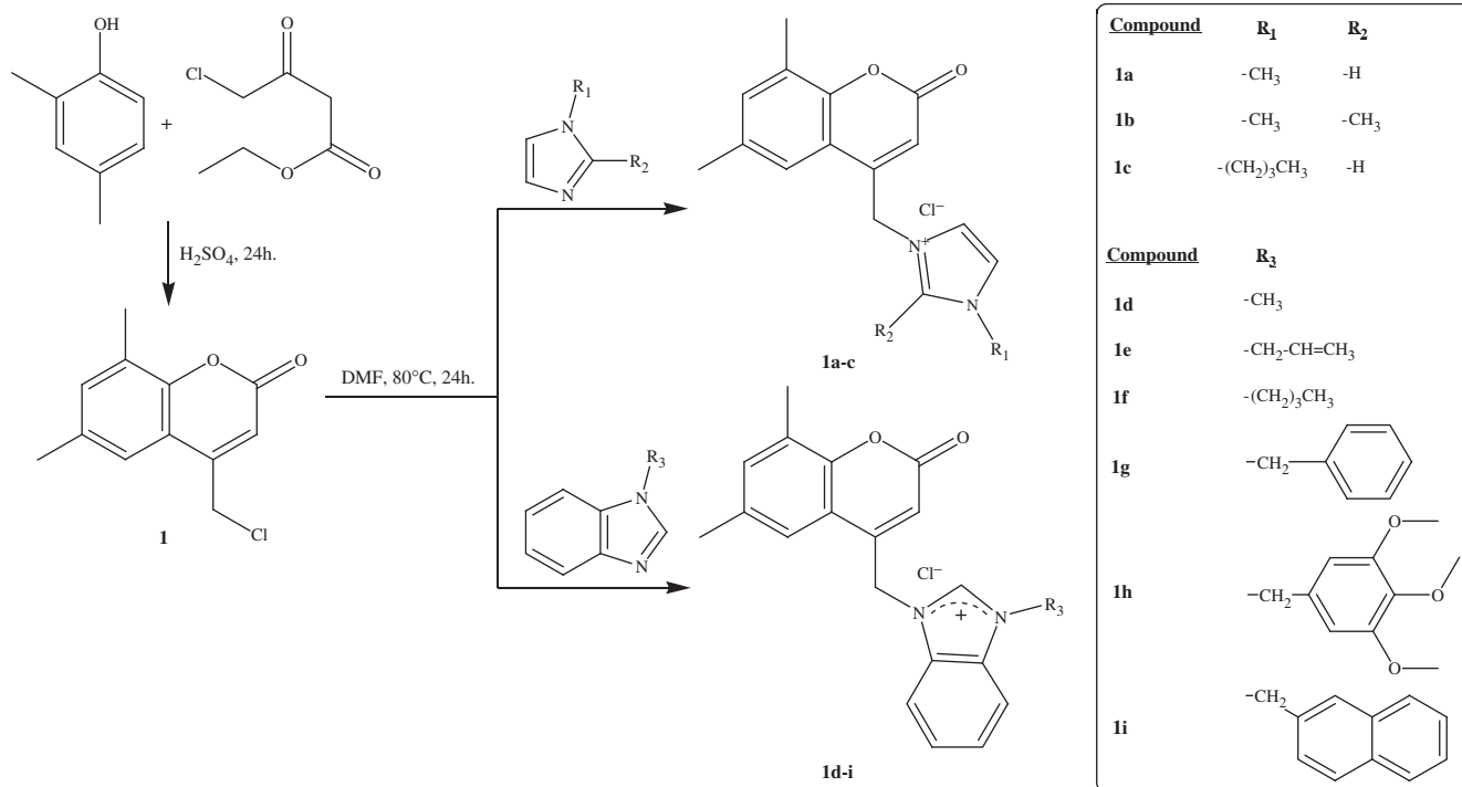
Scheme 1. Synthesis of 6,8-dimethyl coumarin bearing imidazolium and benzimidazolium salts ( 1a-i ).
