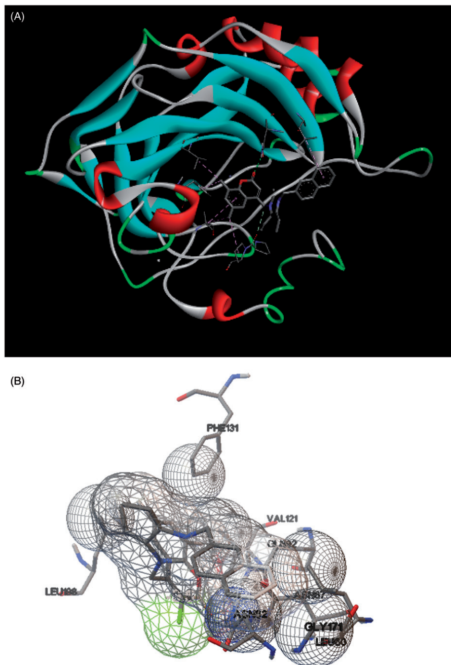
Figure 2. Docking of compound 1i within the hCA II active site. (A) Discovery Studio 4.0 Client images and (B) ADT images.
