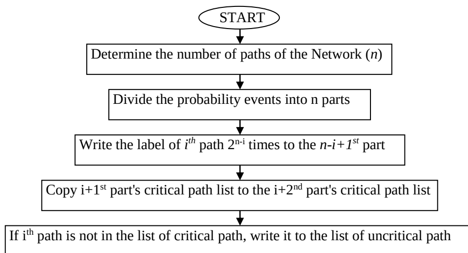
Figure 3. Flowchart of the cloning algorithm
