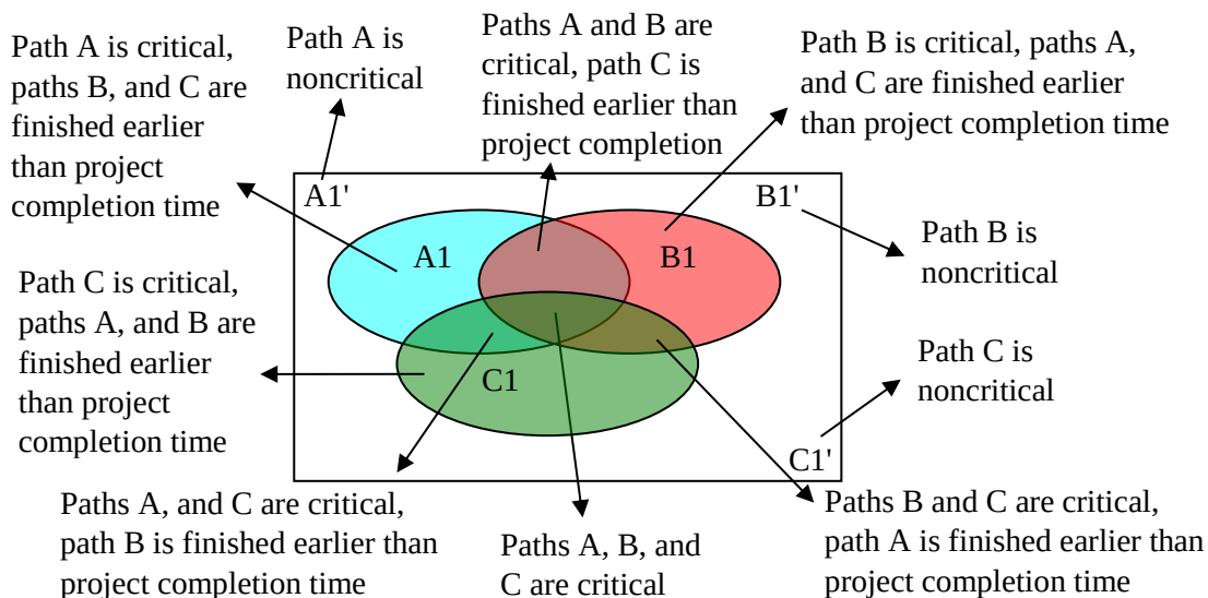
Figure 2. Possibilities of critical paths if the network has three paths
