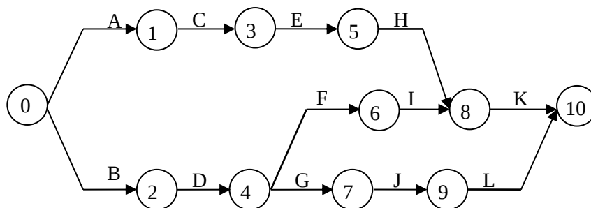
Figure 5. Activity on arrow diagram of the second problem
