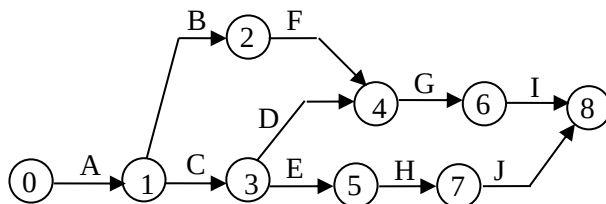
Figure 4. Activity on arrow diagram of the first problem
