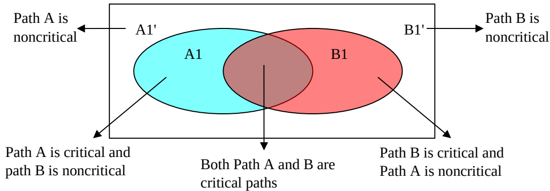
Figure 1. Possible events are shown by shaded areas in case of two paths
