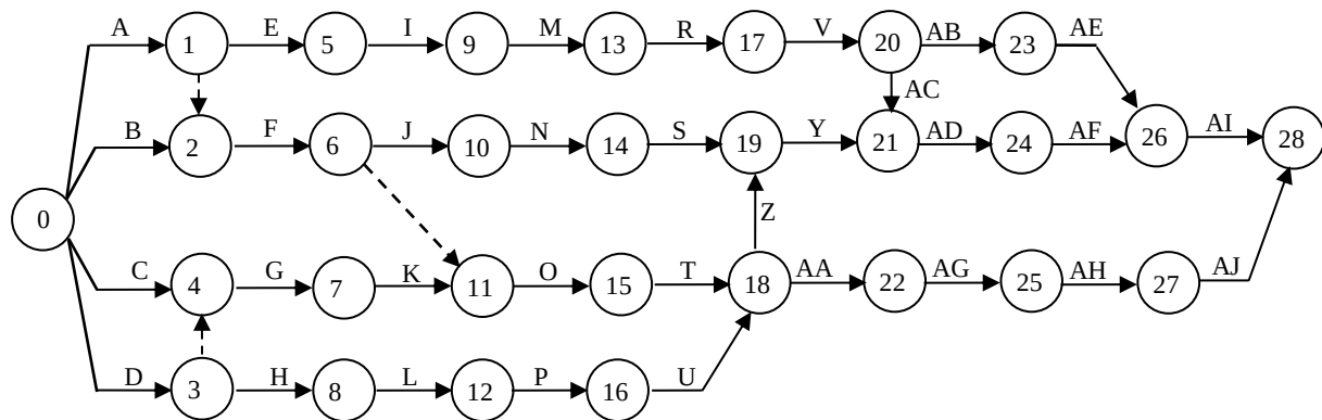
Figure 7. Activity on arrow diagram of the fifth problem
