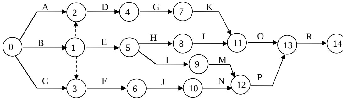
Figure 6. Activity on arrow diagram of the third problem
