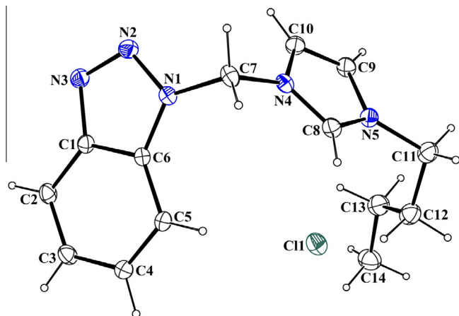
Figure 2. A view of compound 2c showing the atom-numbering scheme. Displacement ellipsoids are drawn at the 10% probability level and H atoms are shown as small spheres of arbitrary radii. For clarity, only the major part of the disordered butyl moiety is shown.
