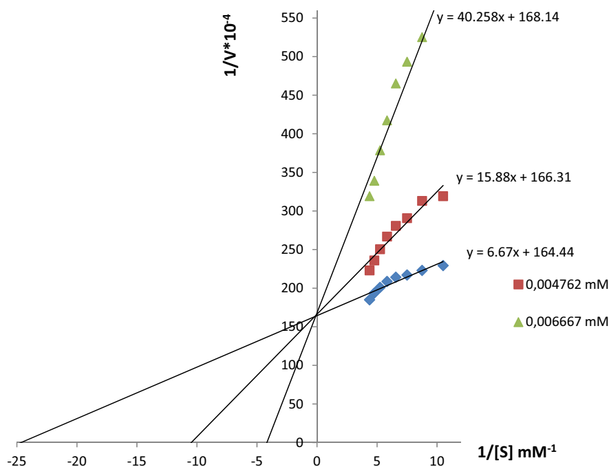
Figure 3. Inhibition of paraoxonase by compound 1c . The slope of Lineweaver–Burk plots indicates competitive inhibition for paraoxon.
