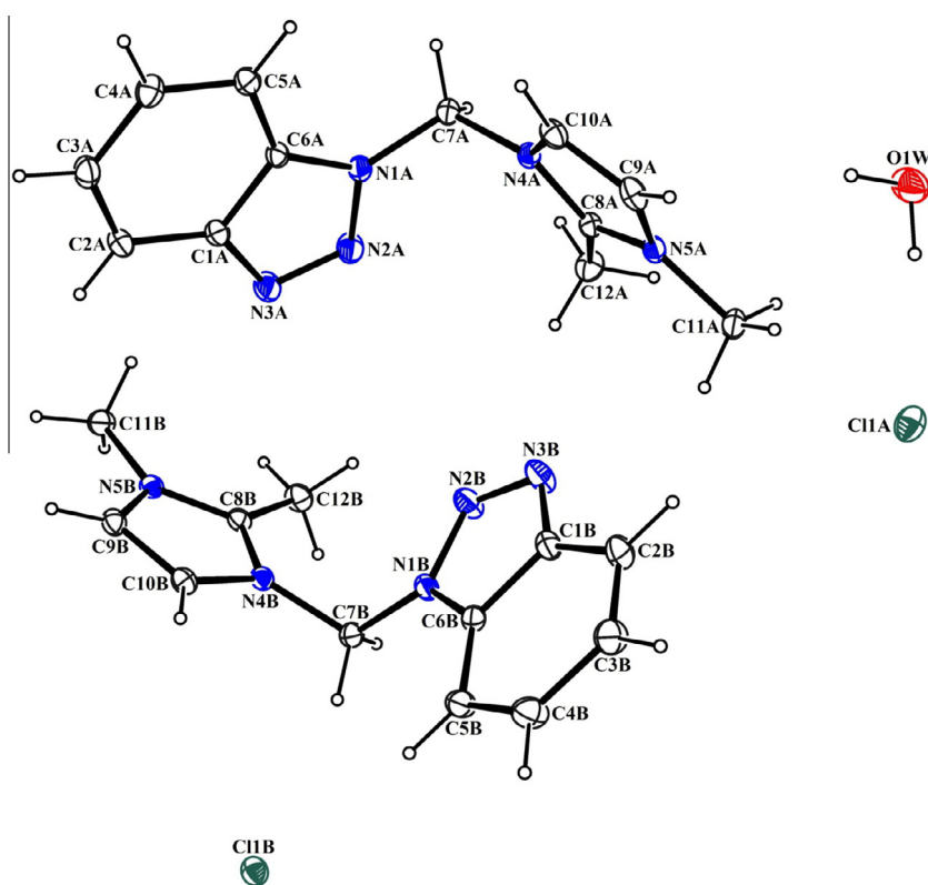
Figure 1. A view of compound 2b showing the atom-numbering scheme. Displacement ellipsoids are drawn at the 10% probability level and H atoms are shown as small spheres of arbitrary radii.
