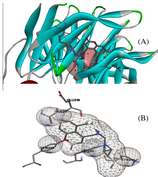
Figure 4. Docking of compound 1c within the active site of PON1 (A) Discovery Studio 4.0 Client images and (B) ADT images.
