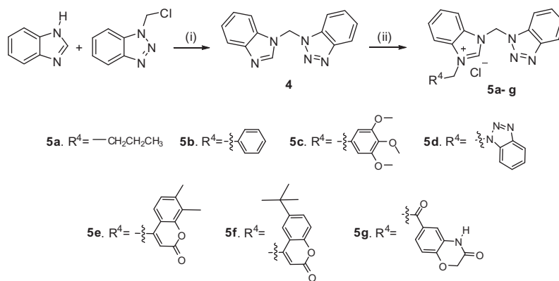
Scheme 3. Synthesis and structures of benzimidazolium salts. Reagents and conditions: (i) KOH, EtOH, reflux, 24 h, (ii) R^4CH_2Cl , DMF, 90 °C, 8 h.
