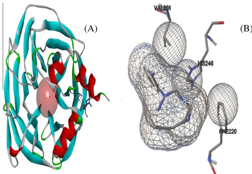
Figure 5. Docking of compound 2c within the active site of PON1 (A) Discovery Studio 4.0 Client images and (B) ADT images.
