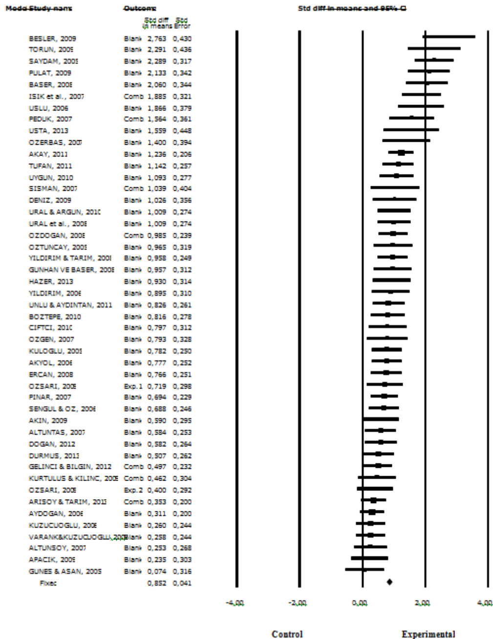
Graph 2. Forest plot of the studies
